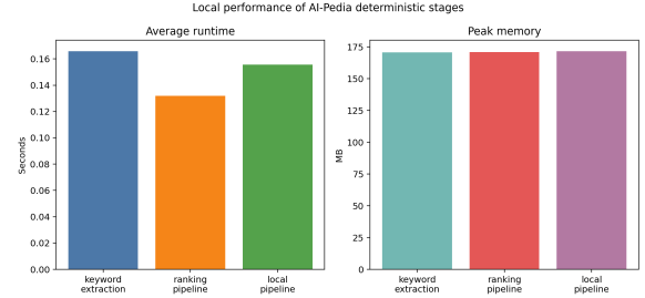
Fig. 10. Runtime and peak memory for deterministic local stages.
